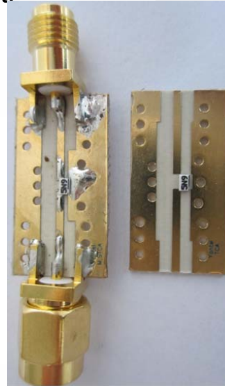
Evaluation board
