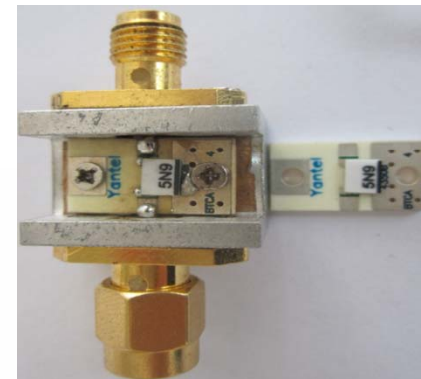
Test fixture
