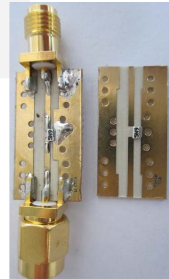
Test fixture
