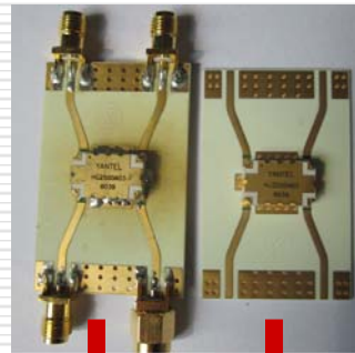
Test fixture Eval board
