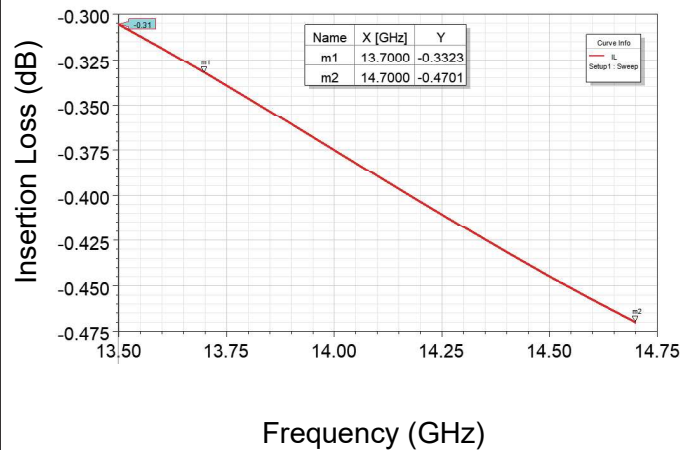
Insertion Loss (Port 1 feeding)
