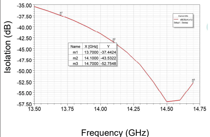
Isolation (Port 1 feeding)
