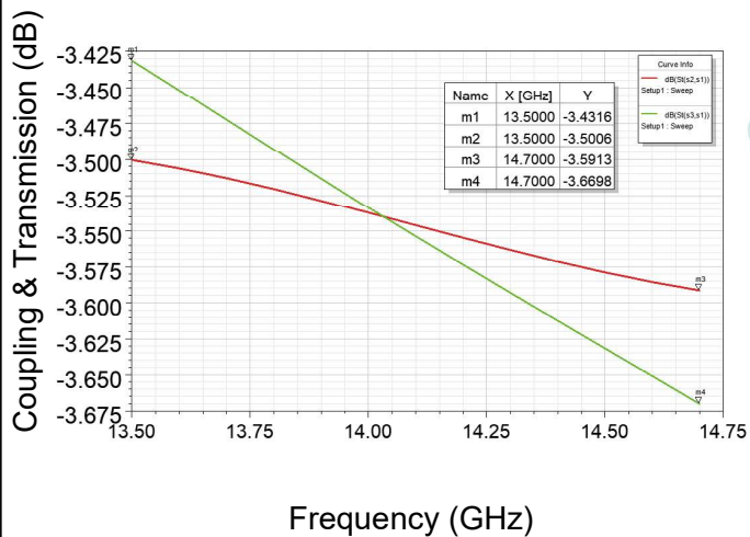
Coupling & Transmission (Port 1 feeding)
