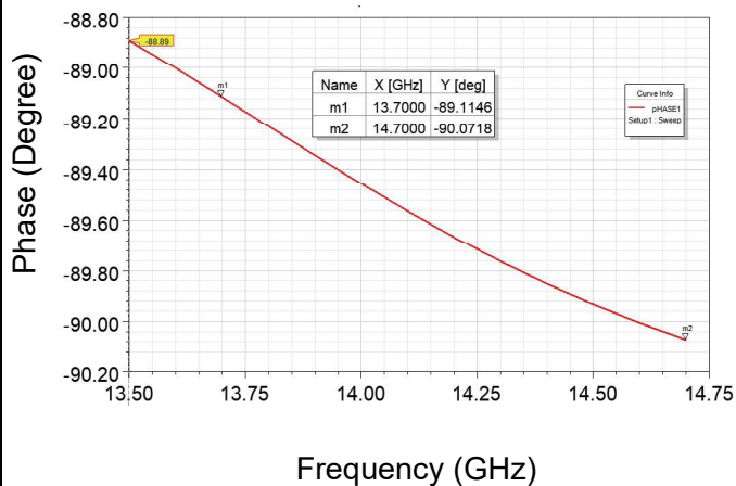
Phase (Port 1 feeding)
