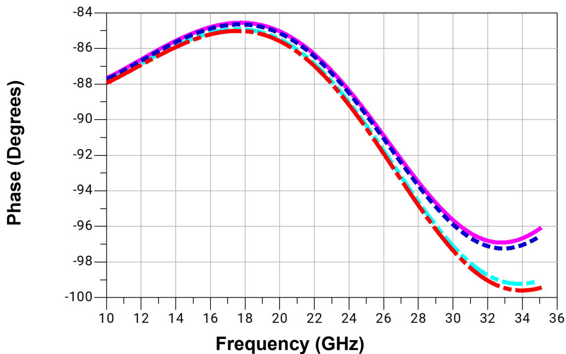
Phase Balance VS.Frequency
