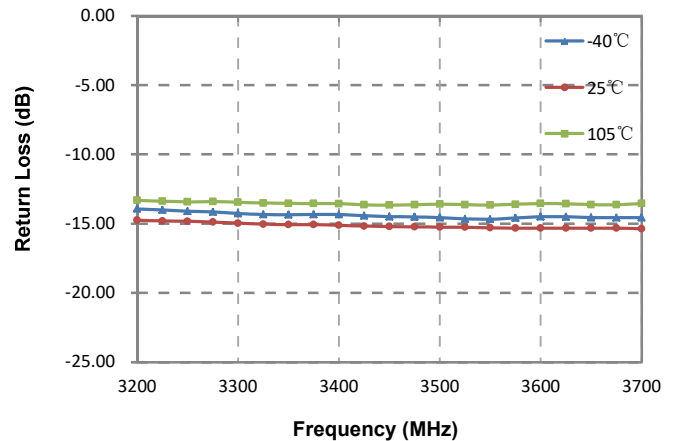
Return Loss (Port 4)
