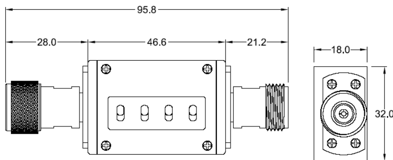
Package type: N22, Net weight: 78.8 g
