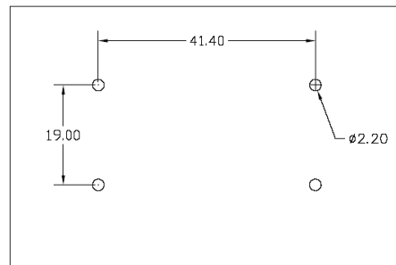
Mounting holes on user's panel Fig 6
