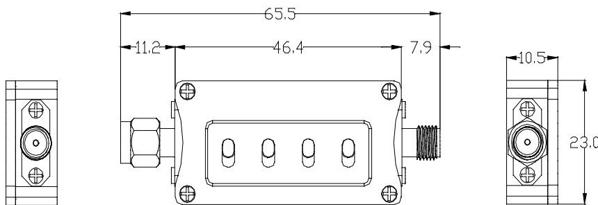
Package type: S22, Net weight: 24.3g
