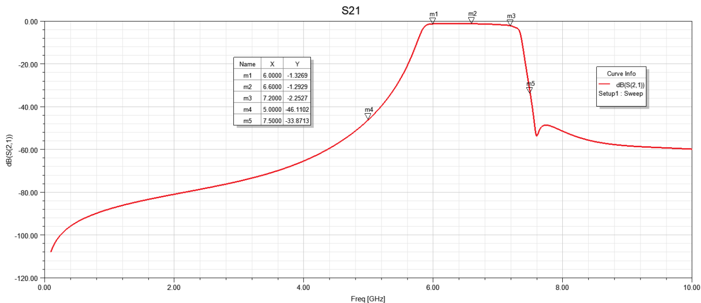
Insertion Loss-S21
