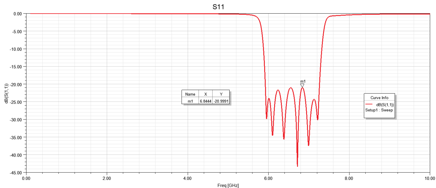
Return Loss -S11
