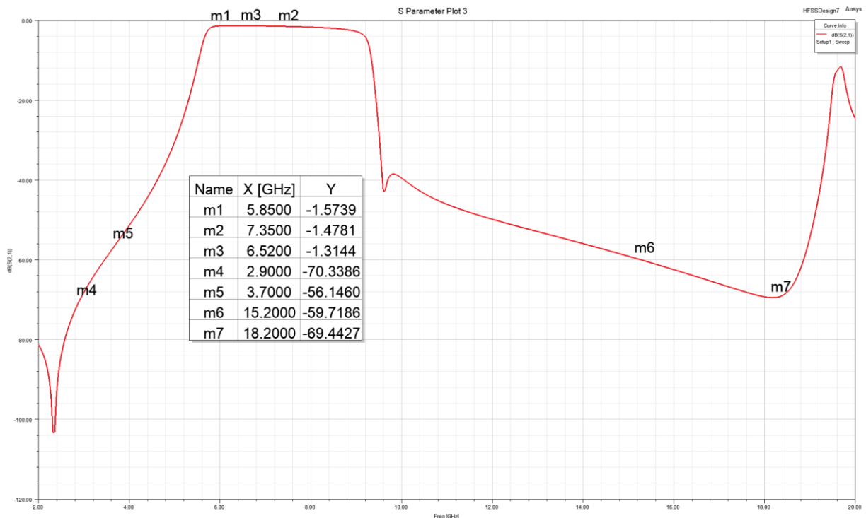
Insertion Loss-S21
