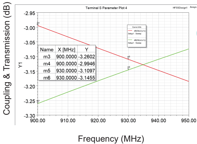
Coupling & Transmission (Port 1 feeding)
