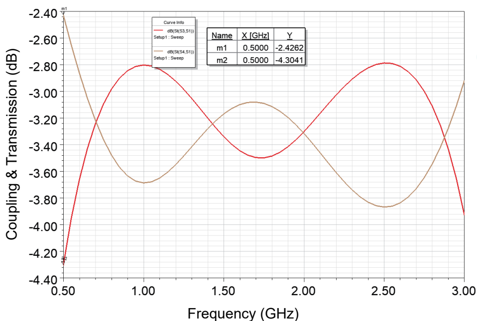
Coupling & Transmission (Port 1 feeding)
