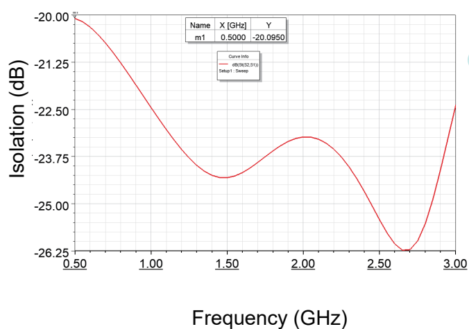
Isolation (Port 1 feeding)
