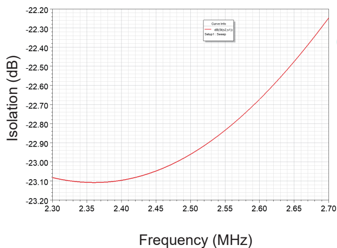
Isolation (Port 1 feeding)
